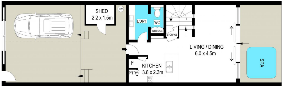
GROUND FLOOR
