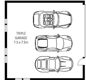
GARAGING
